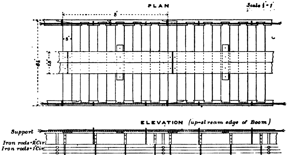
Fig. 265.—Dagpathar boom.
